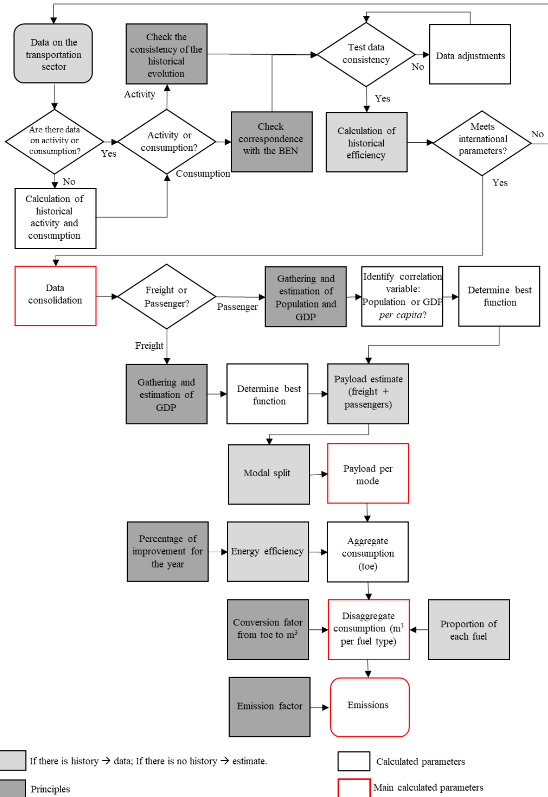
Figure A-1. Procedure adopted to estimate energy consumption using the top-down approach.
